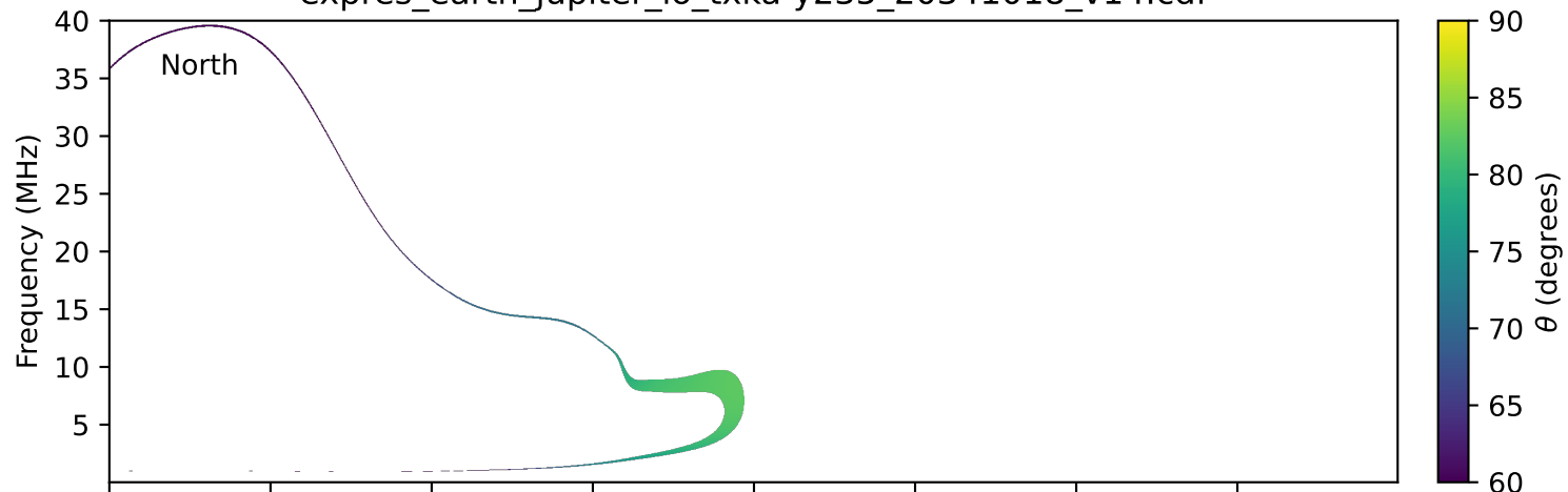
expres_earth_jupiter_io_txka-y235_20341018_v14.cdf
