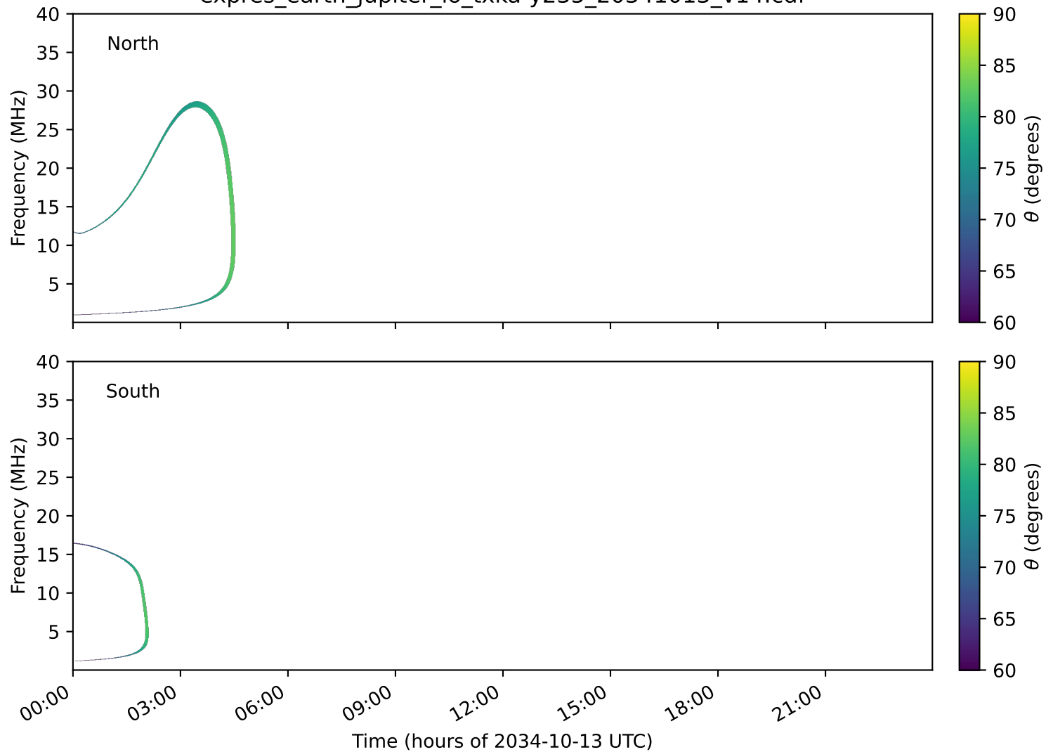
expres_earth_jupiter_io_txka-y235_20341013_v14.cdf
