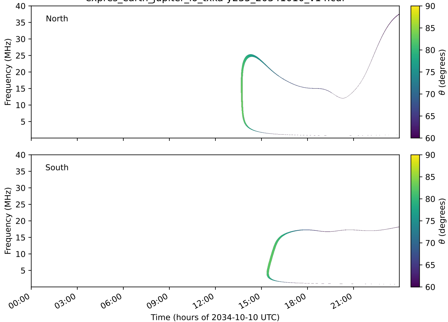
expres_earth_jupiter_io_txka-y235_20341010_v14.cdf
