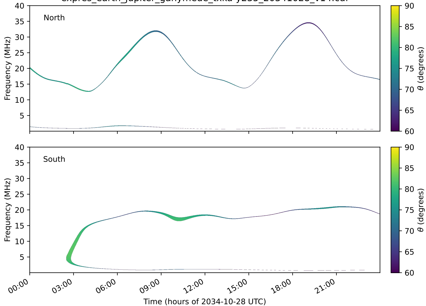
expres_earth_jupiter_ganymede_txka-y235_20341028_v14.cdf
