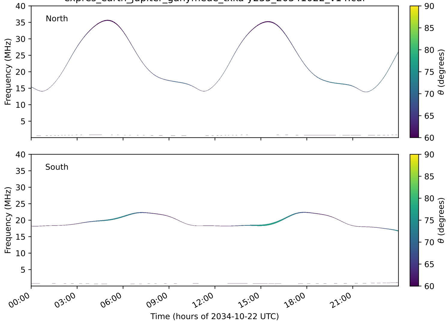
expres_earth_jupiter_ganymede_txka-y235_20341022_v14.cdf
