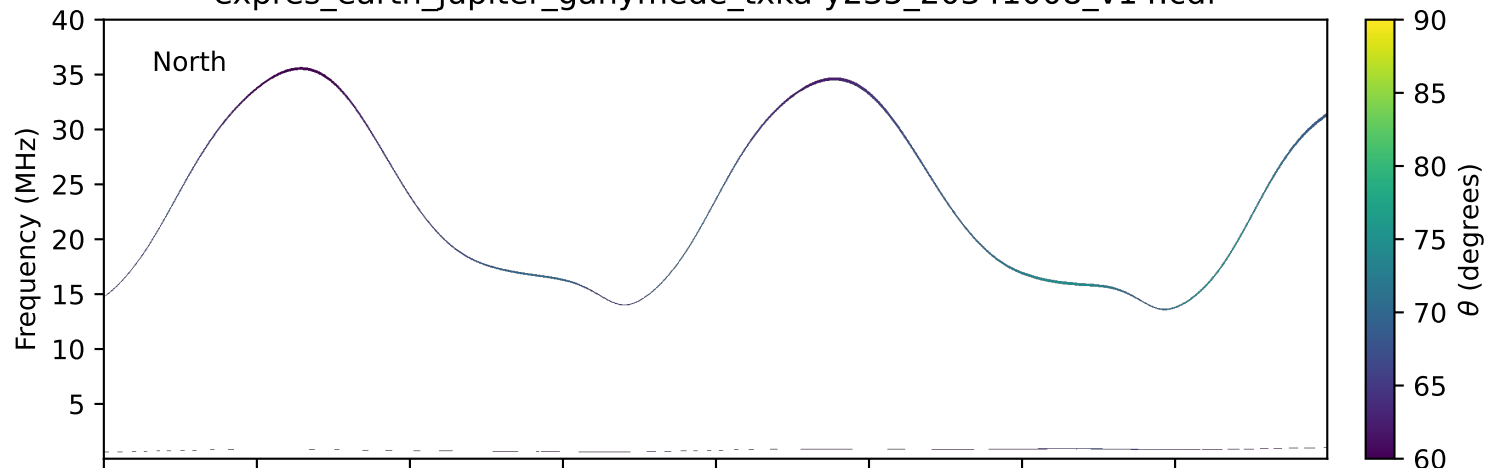
expres_earth_jupiter_ganymede_txka-y235_20341008_v14.cdf
