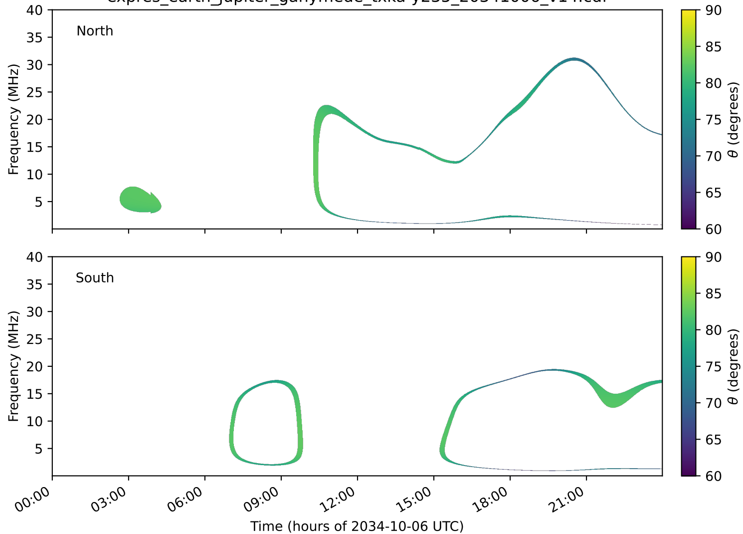
expres_earth_jupiter_ganymede_txka-y235_20341006_v14.cdf
