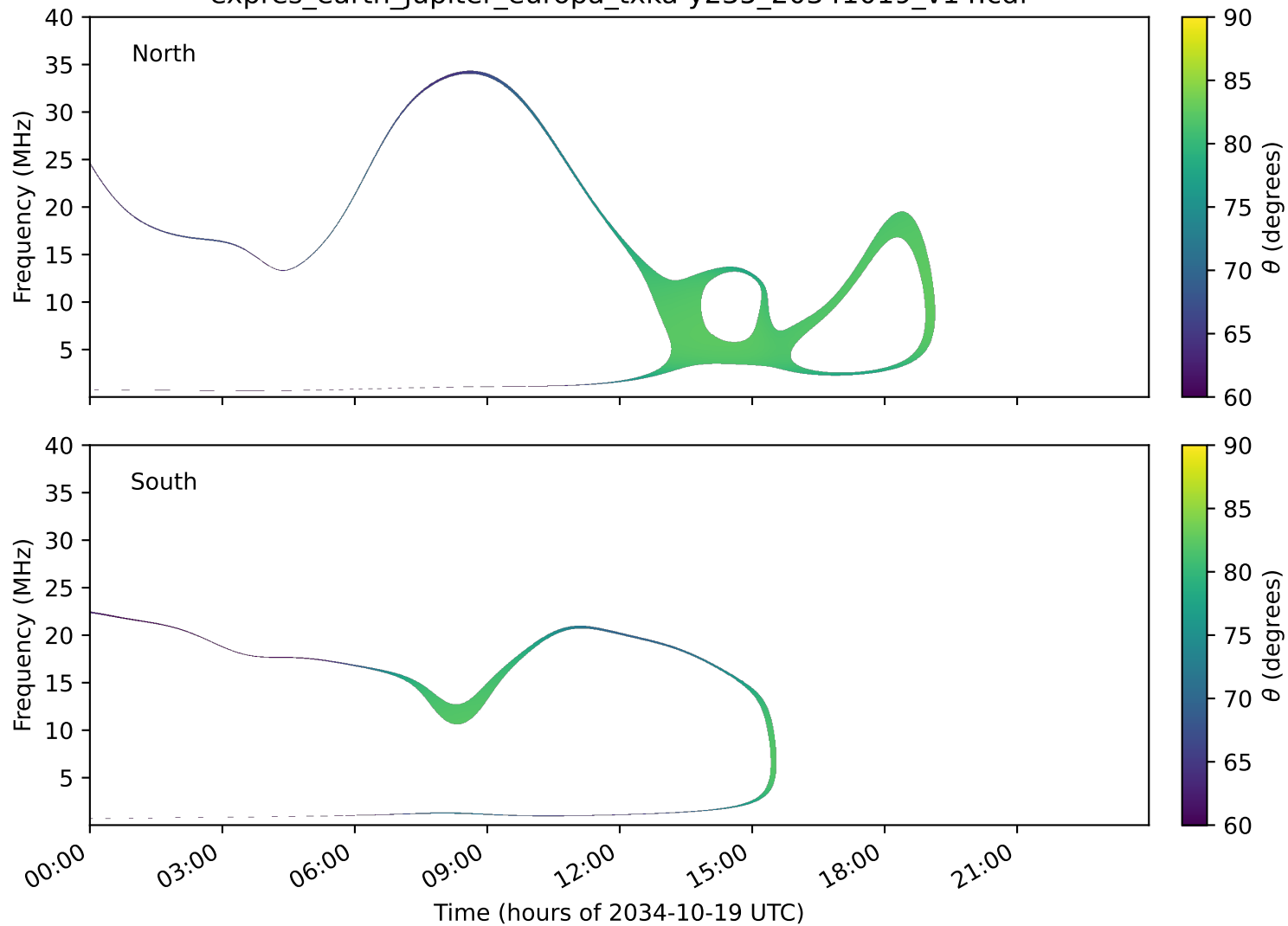
expres_earth_jupiter_europa_txka-y235_20341019_v14.cdf
