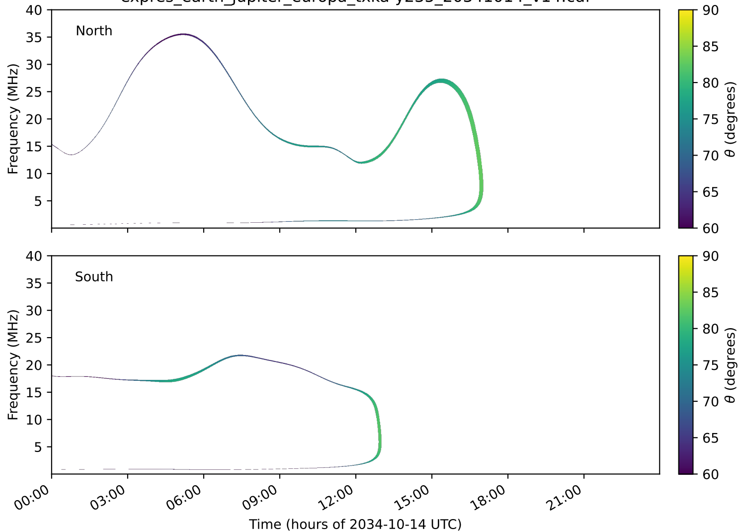
expres_earth_jupiter_europa_txka-y235_20341014_v14.cdf
