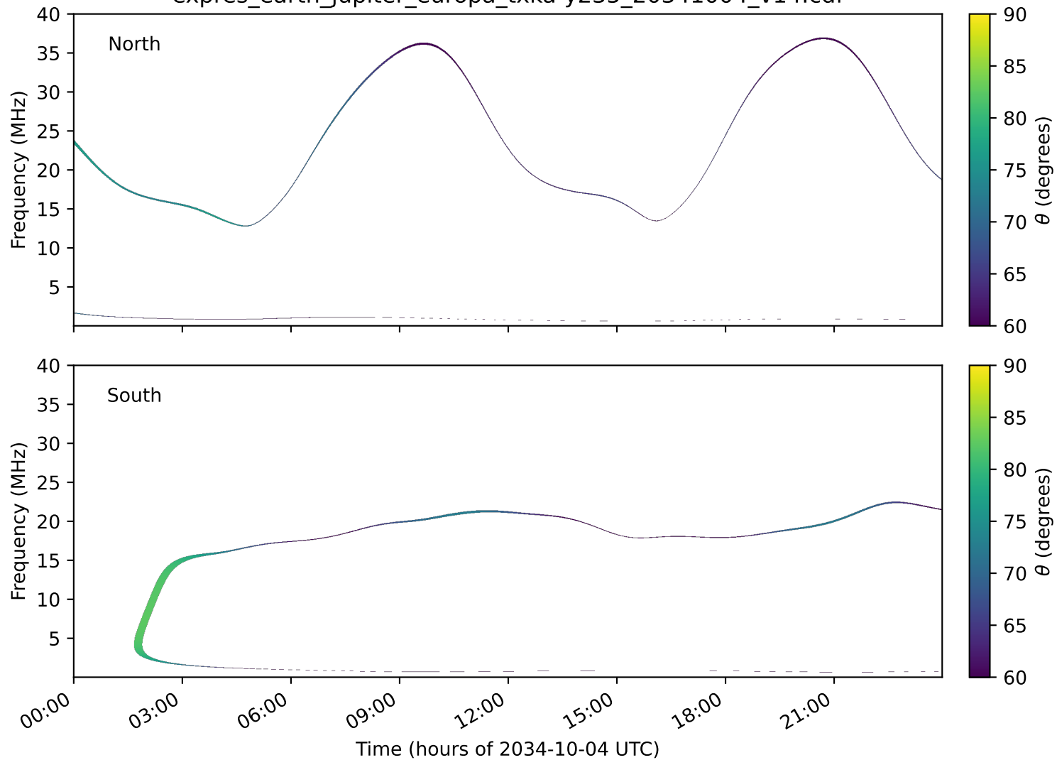
expres_earth_jupiter_europa_txka-y235_20341004_v14.cdf
