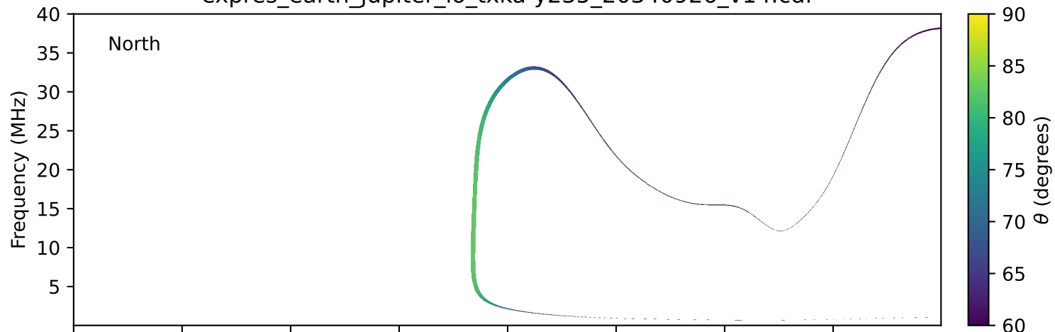
expres_earth_jupiter_io_txka-y235_20340926_v14.cdf
