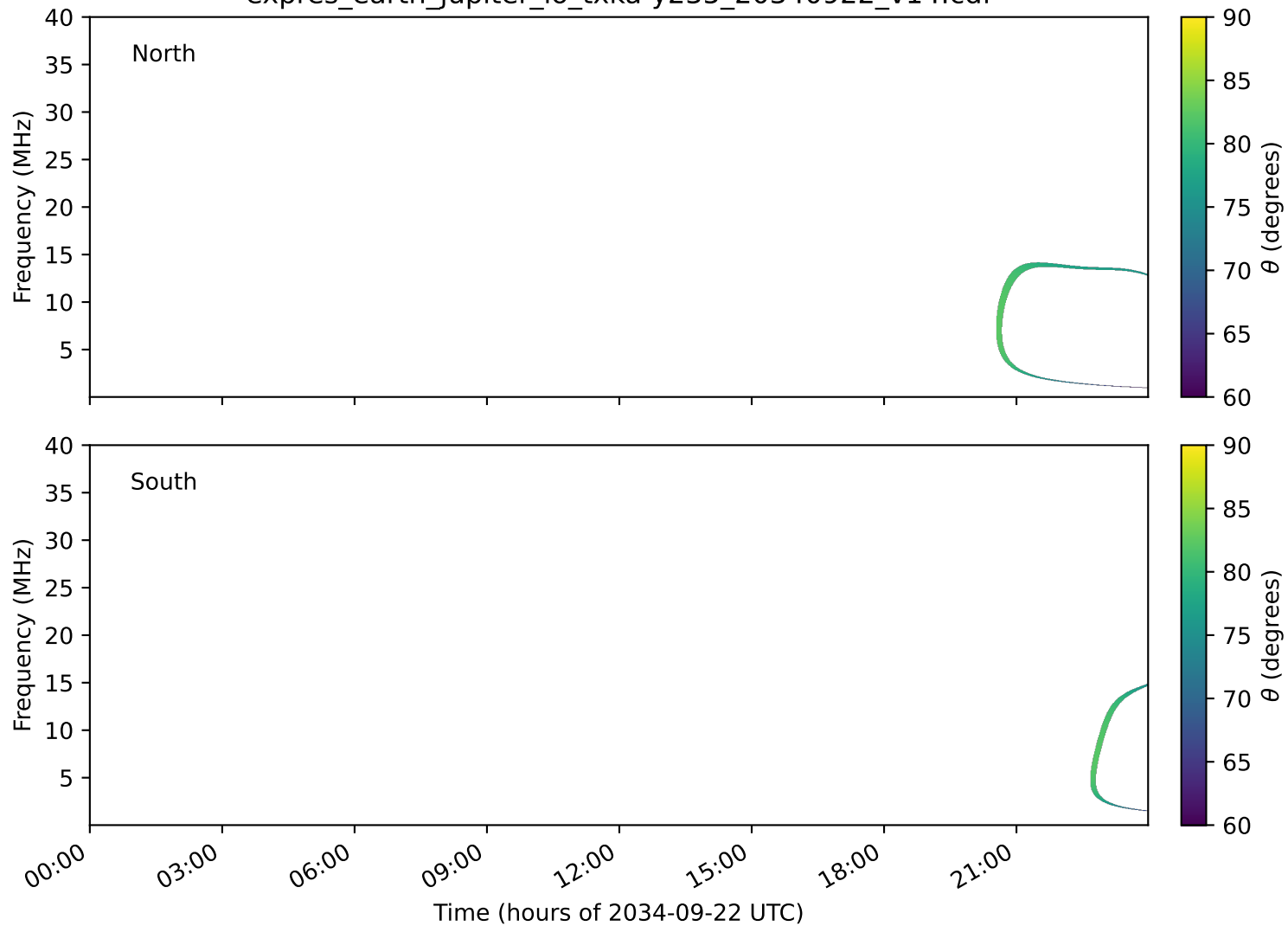
expres_earth_jupiter_io_txka-y235_20340922_v14.cdf
