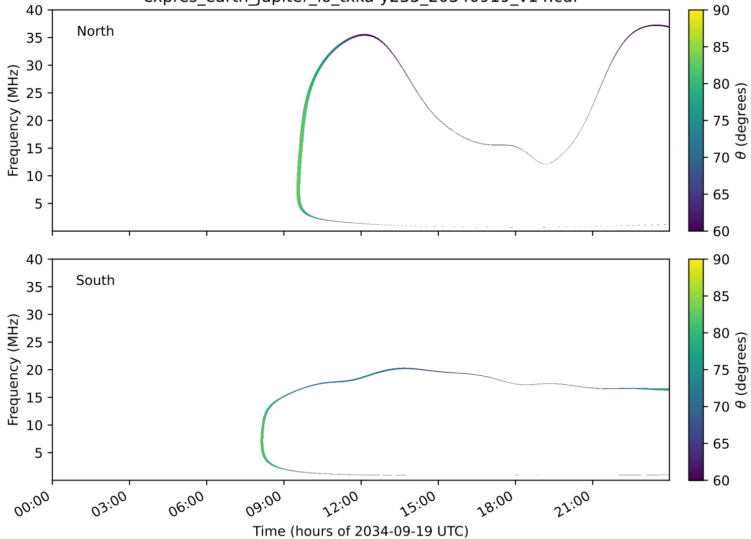
expres_earth_jupiter_io_txka-y235_20340919_v14.cdf
