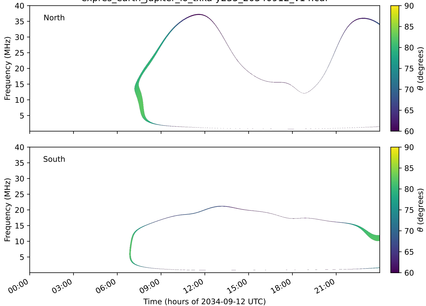
expres_earth_jupiter_io_txka-y235_20340912_v14.cdf
