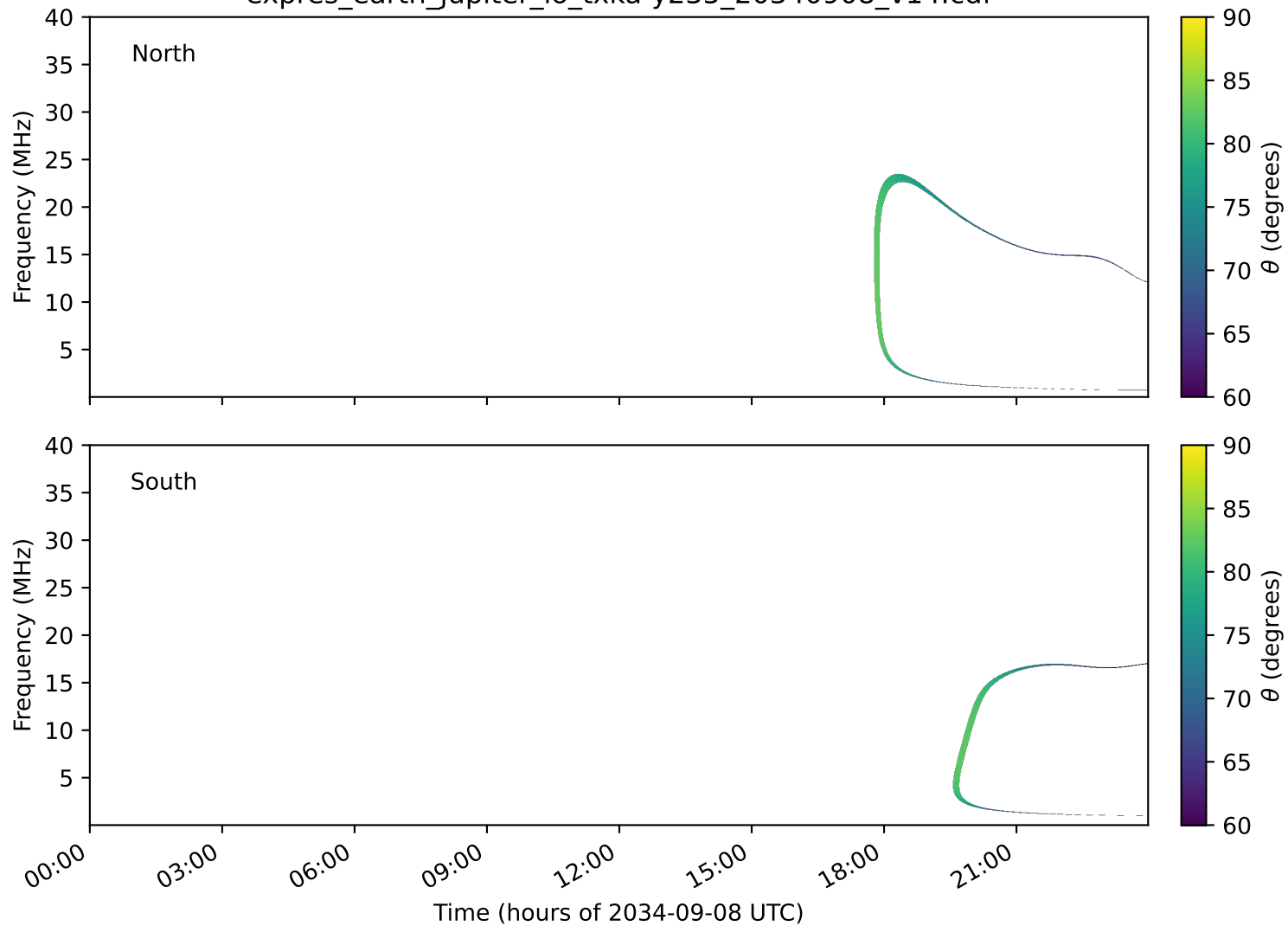
expres_earth_jupiter_io_txka-y235_20340908_v14.cdf
