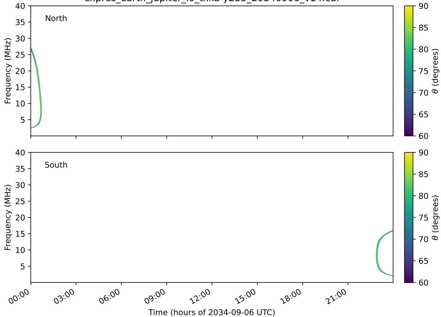
expres_earth_jupiter_io_txka-y235_20340906_v14.cdf
