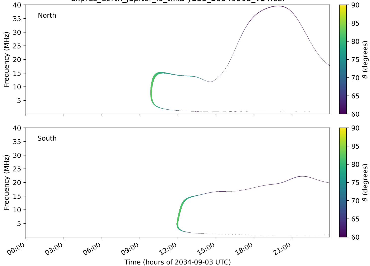
expres_earth_jupiter_io_txka-y235_20340903_v14.cdf
