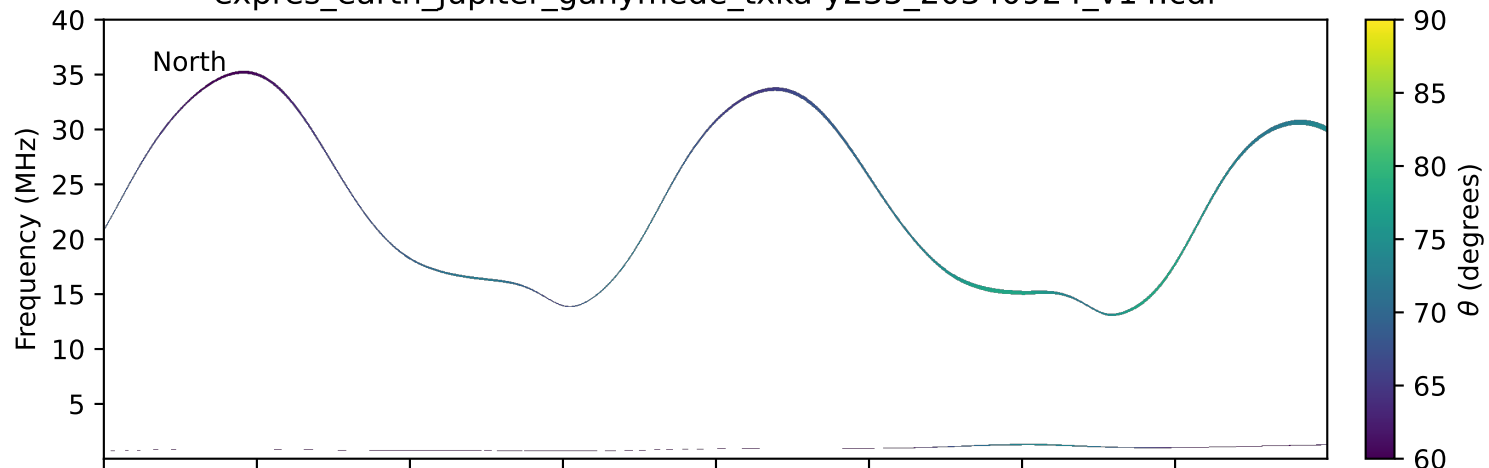
expres_earth_jupiter_ganymede_txka-y235_20340924_v14.cdf
