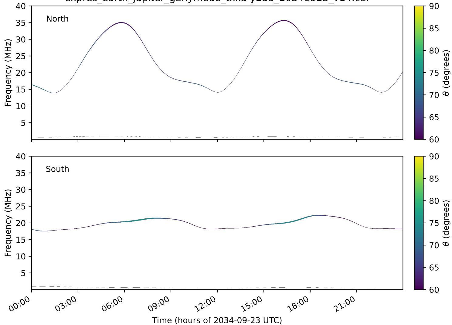
expres_earth_jupiter_ganymede_txka-y235_20340923_v14.cdf
