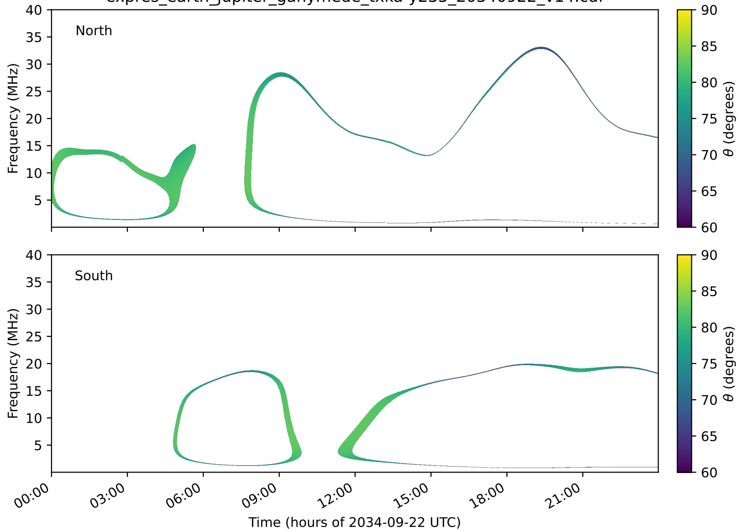
expres_earth_jupiter_ganymede_txka-y235_20340922_v14.cdf
