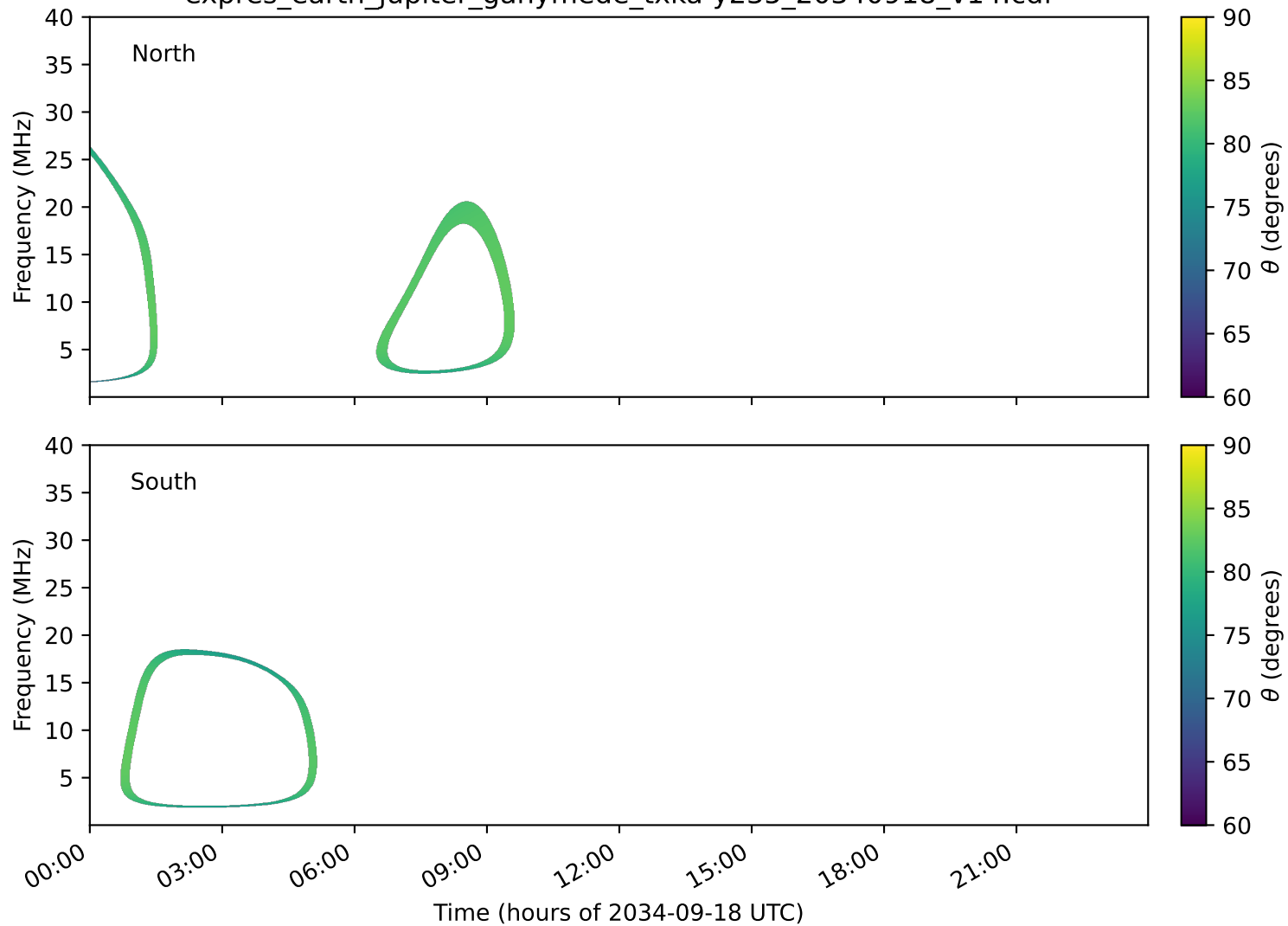
expres_earth_jupiter_ganymede_txka-y235_20340918_v14.cdf
