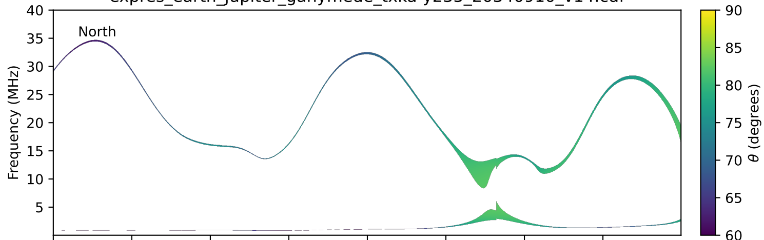
expres_earth_jupiter_ganymede_txka-y235_20340910_v14.cdf
