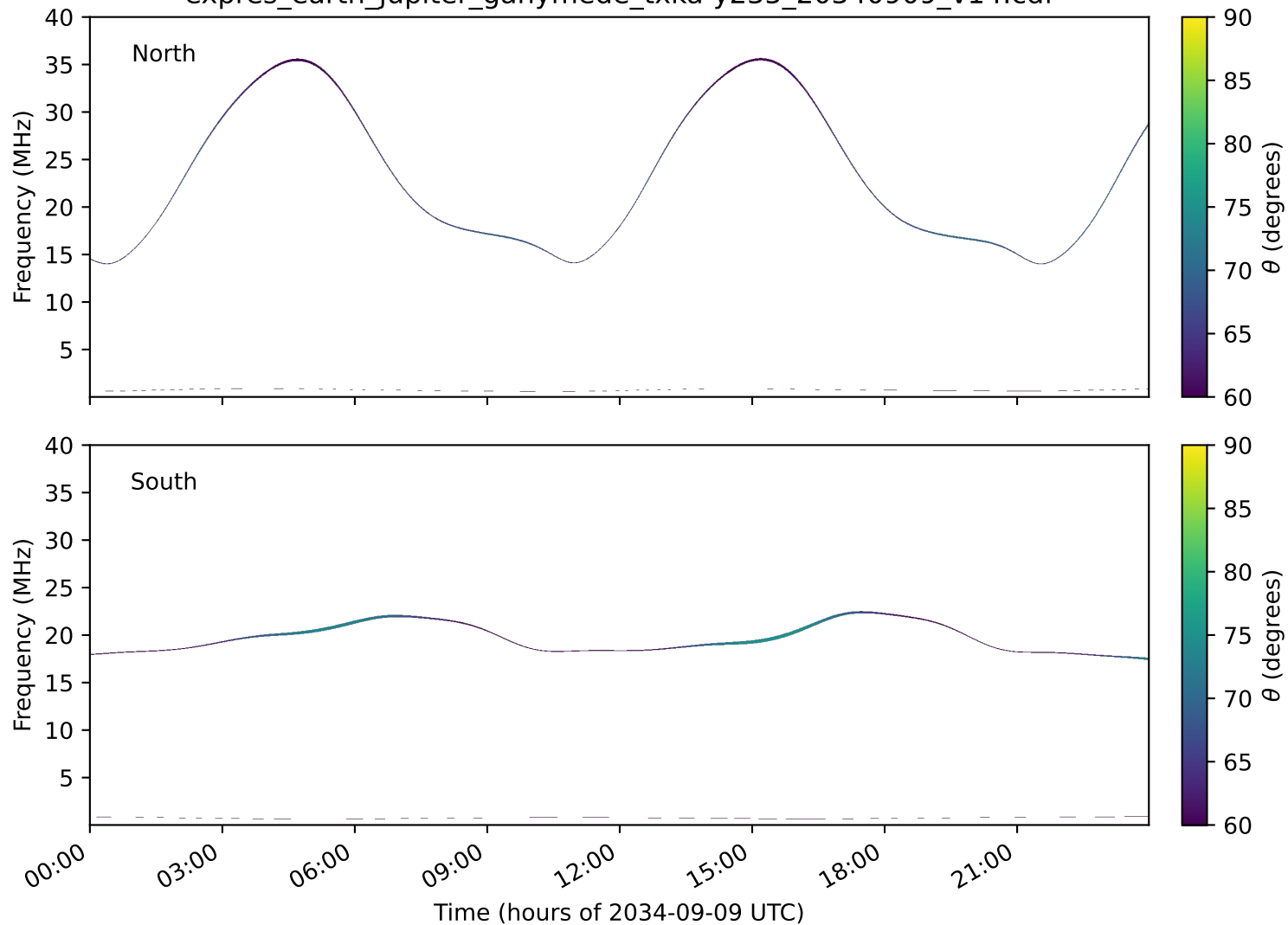
expres_earth_jupiter_ganymede_txka-y235_20340909_v14.cdf
