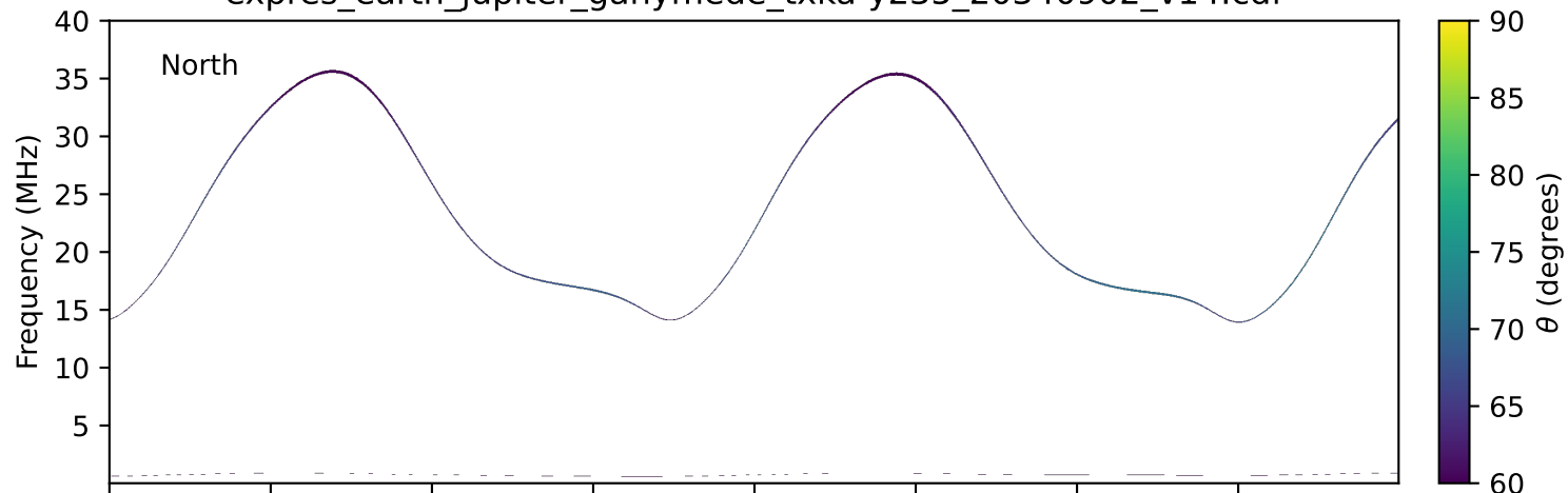
expres_earth_jupiter_ganymede_txka-y235_20340902_v14.cdf
