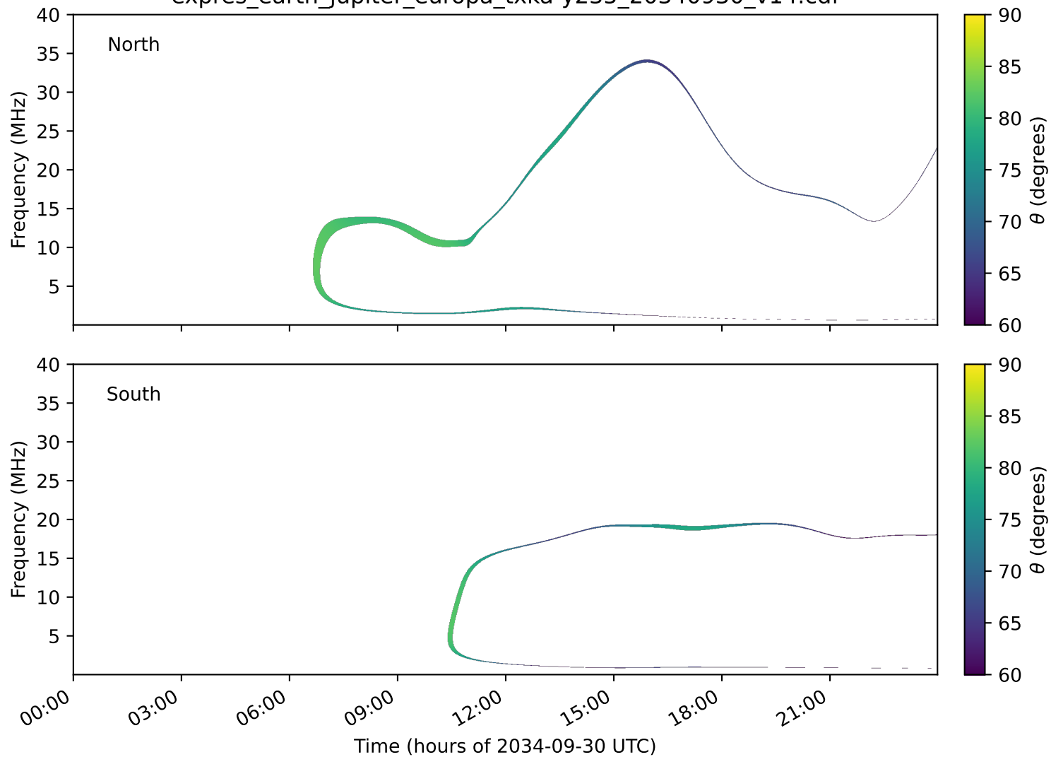
expres_earth_jupiter_europa_txka-y235_20340930_v14.cdf
