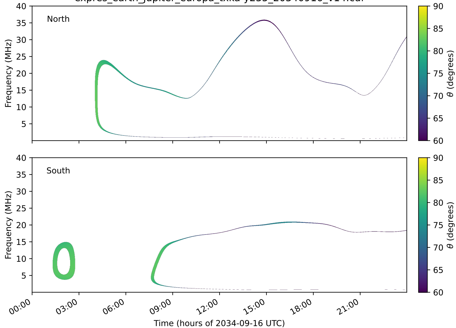
expres_earth_jupiter_europa_txka-y235_20340916_v14.cdf
