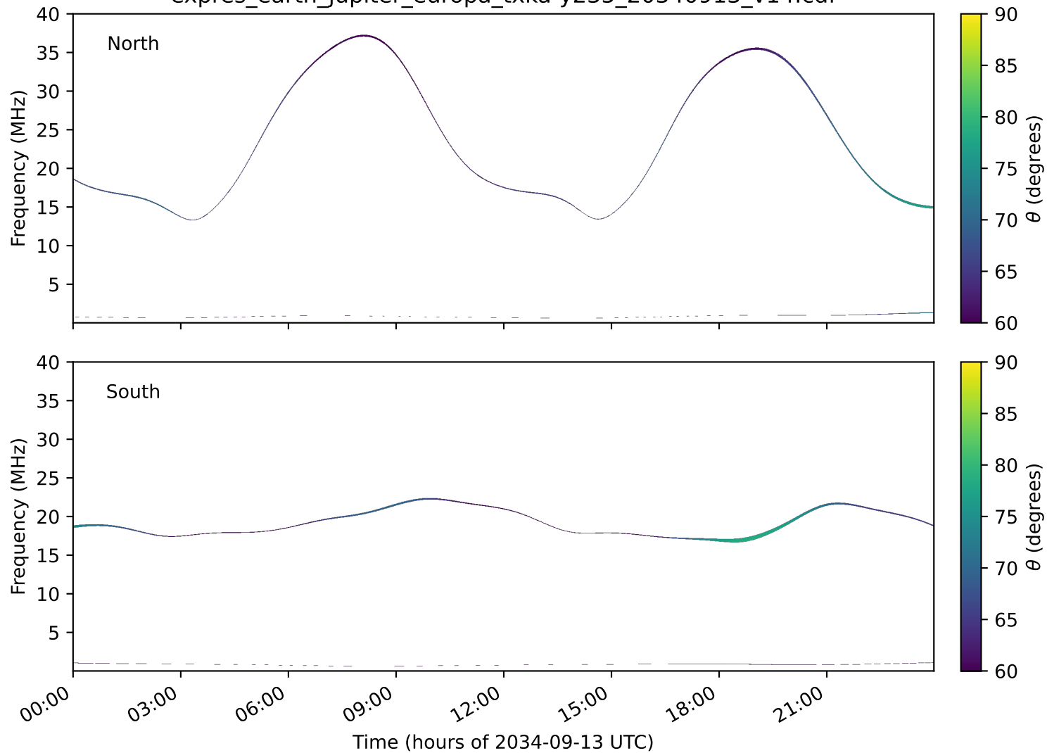
expres_earth_jupiter_europa_txka-y235_20340913_v14.cdf
