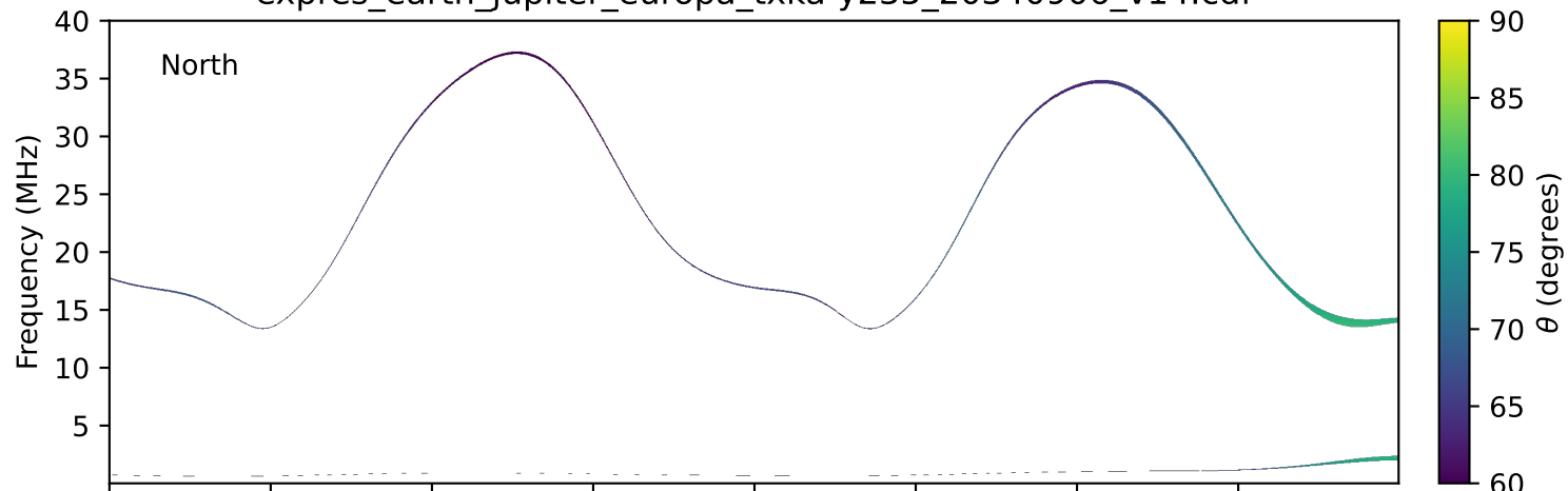
expres_earth_jupiter_europa_txka-y235_20340906_v14.cdf
