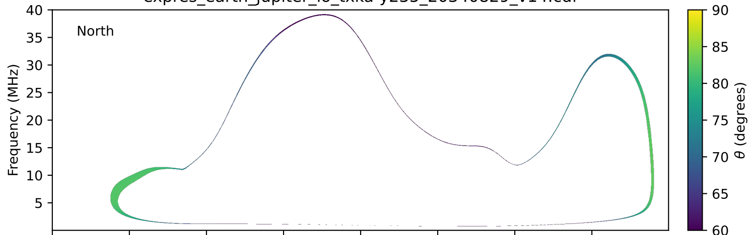
expres_earth_jupiter_io_txka-y235_20340829_v14.cdf
