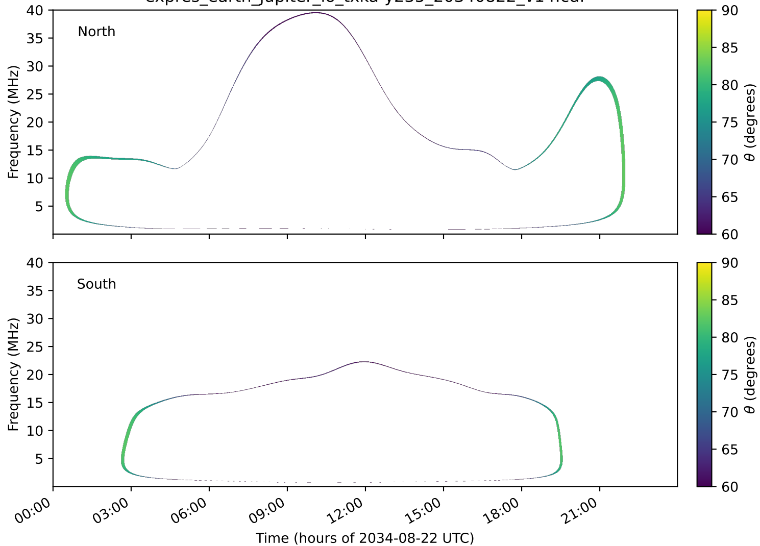
expres_earth_jupiter_io_txka-y235_20340822_v14.cdf
