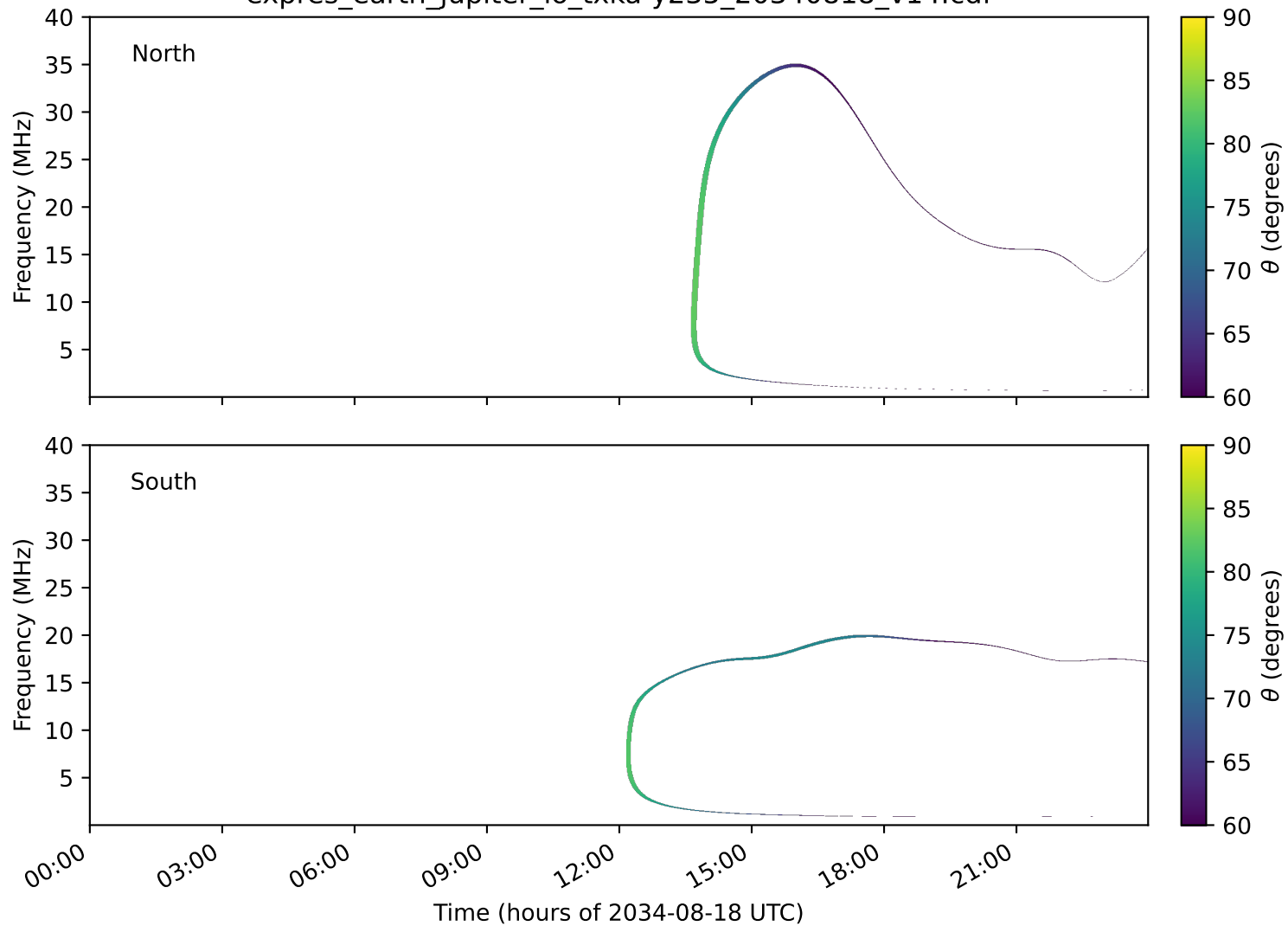
expres_earth_jupiter_io_txka-y235_20340818_v14.cdf
