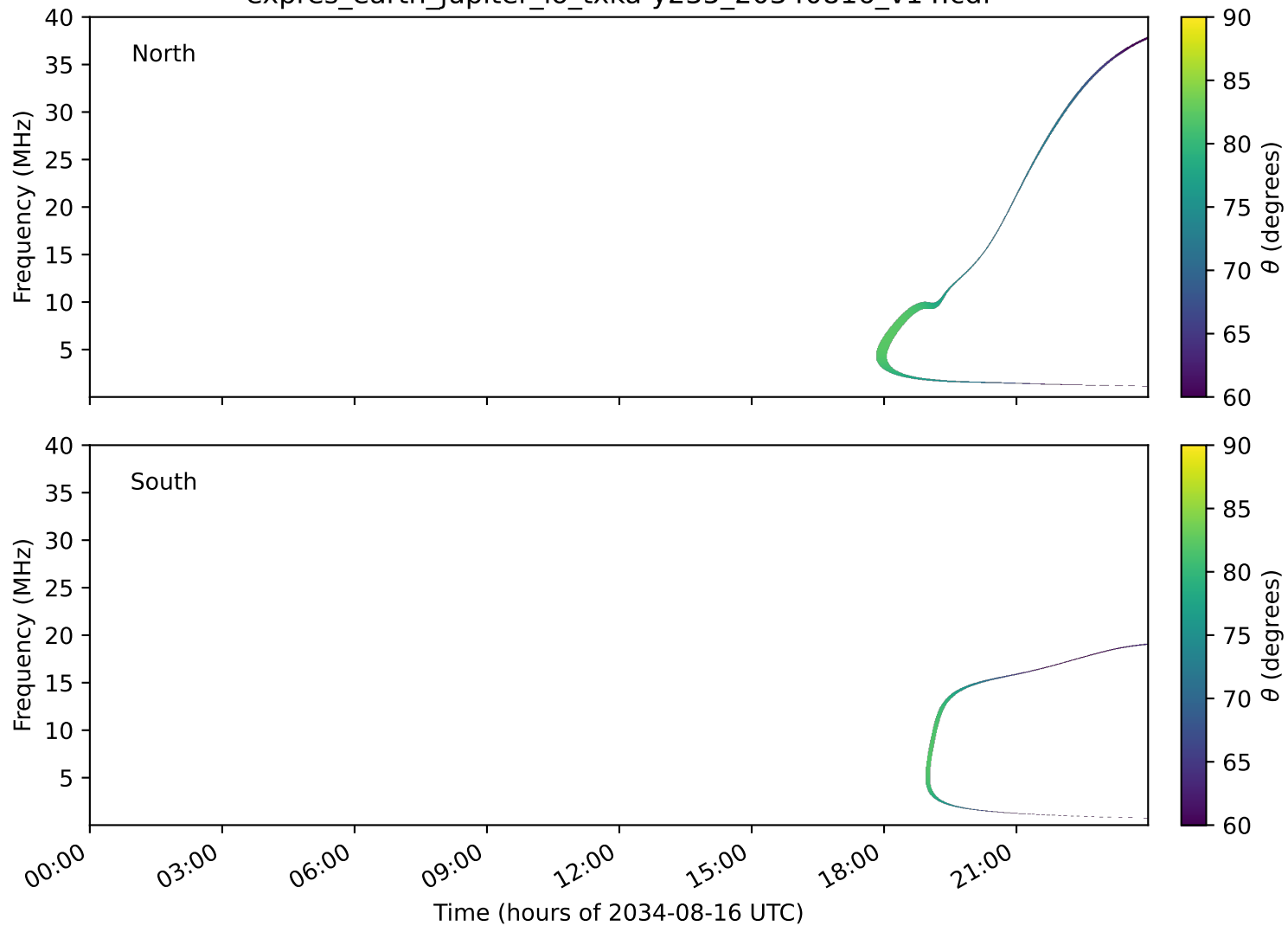
expres_earth_jupiter_io_txka-y235_20340816_v14.cdf
