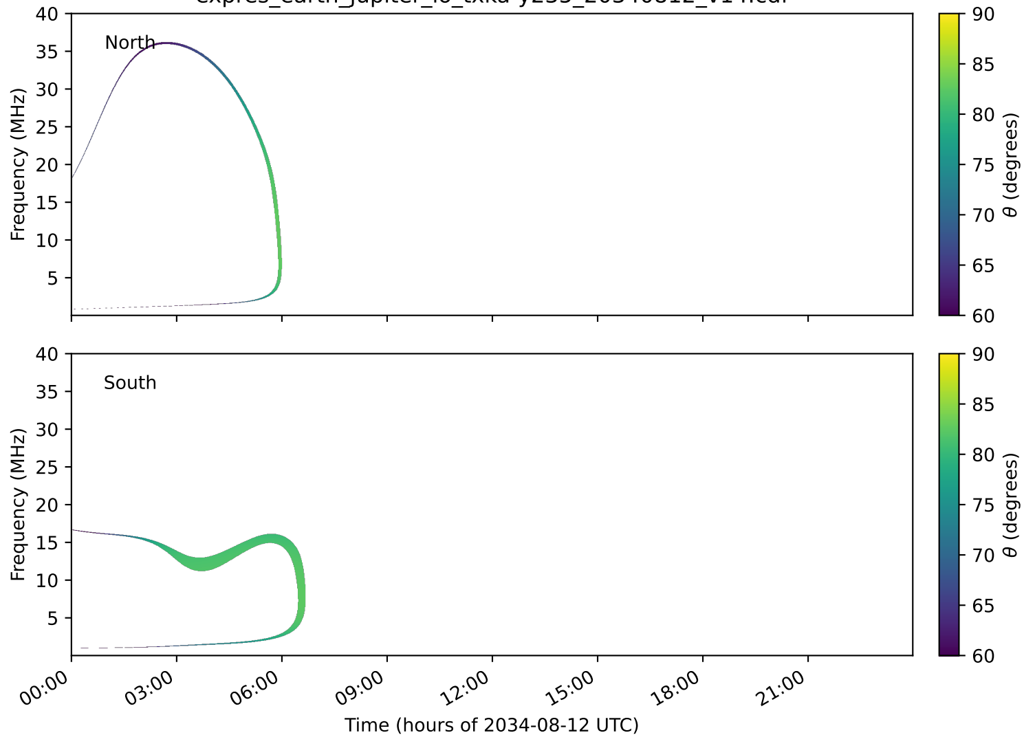
expres_earth_jupiter_io_txka-y235_20340812_v14.cdf
