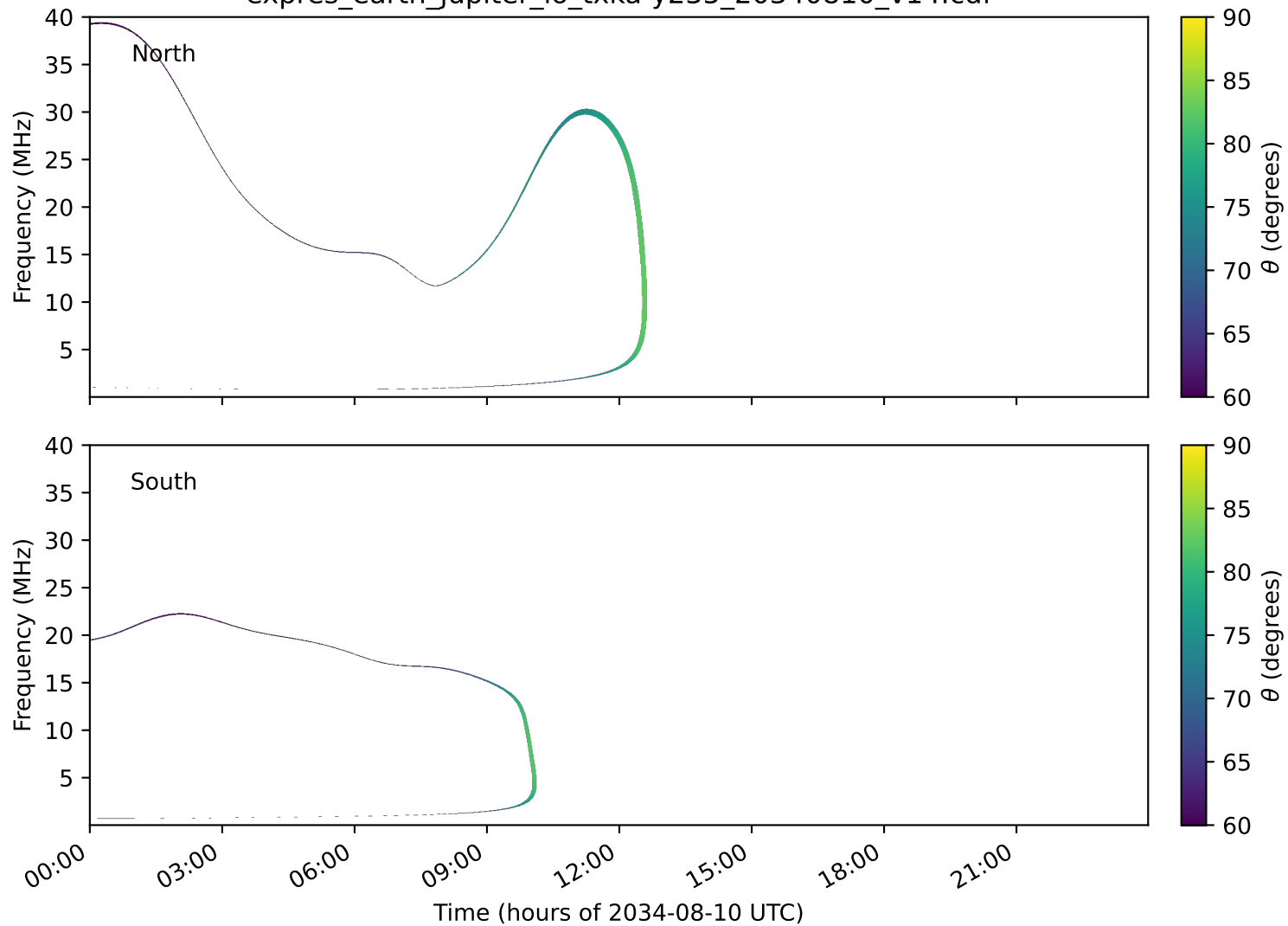
expres_earth_jupiter_io_txka-y235_20340810_v14.cdf
