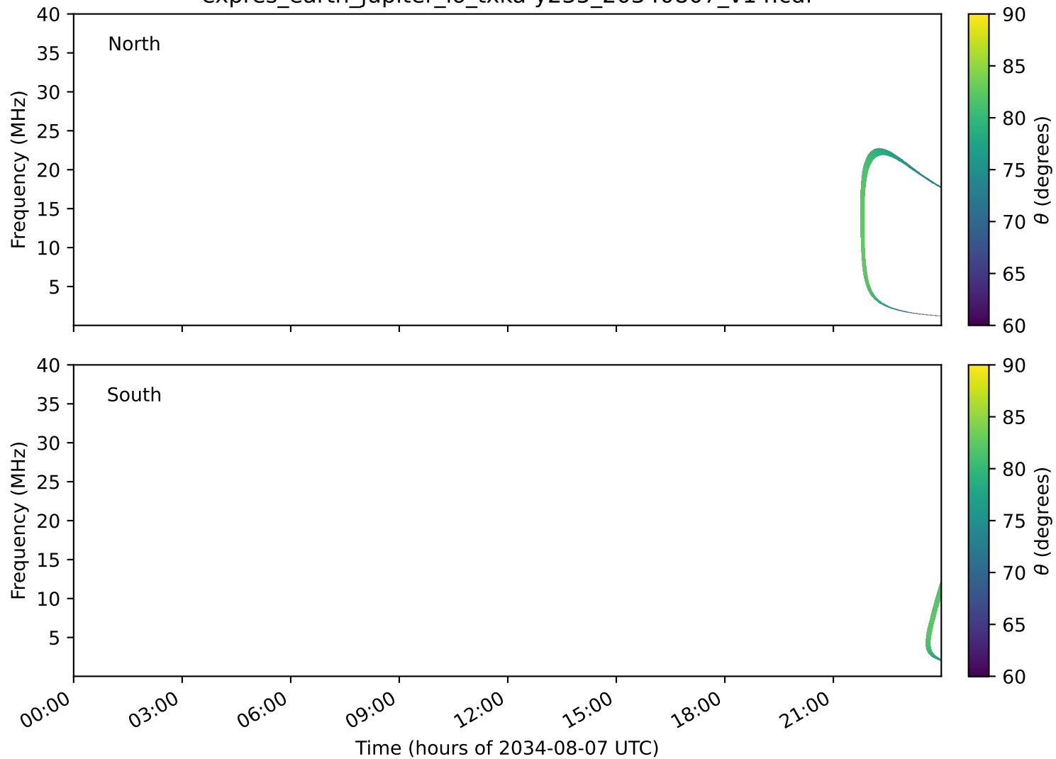
expres_earth_jupiter_io_txka-y235_20340807_v14.cdf
