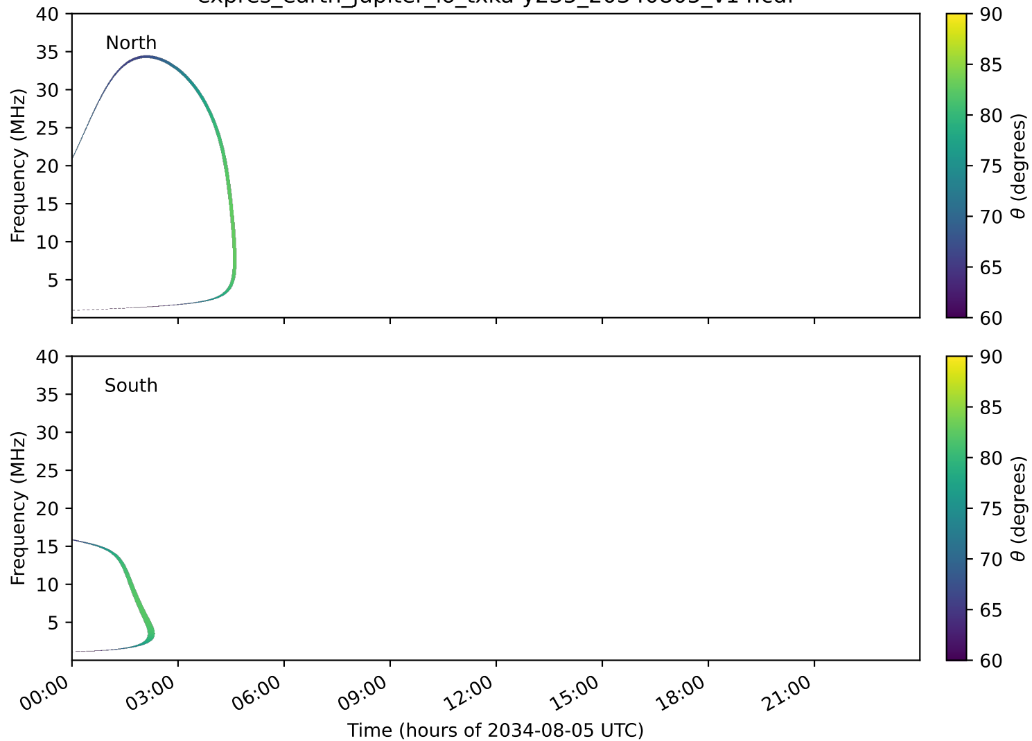
expres_earth_jupiter_io_txka-y235_20340805_v14.cdf
