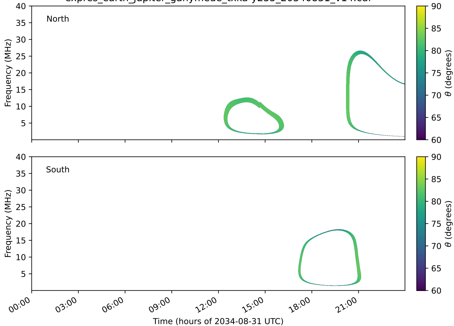
expres_earth_jupiter_ganymede_txka-y235_20340831_v14.cdf
