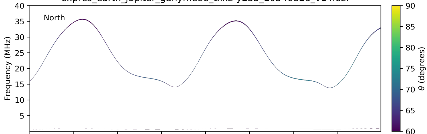
expres_earth_jupiter_ganymede_txka-y235_20340826_v14.cdf
