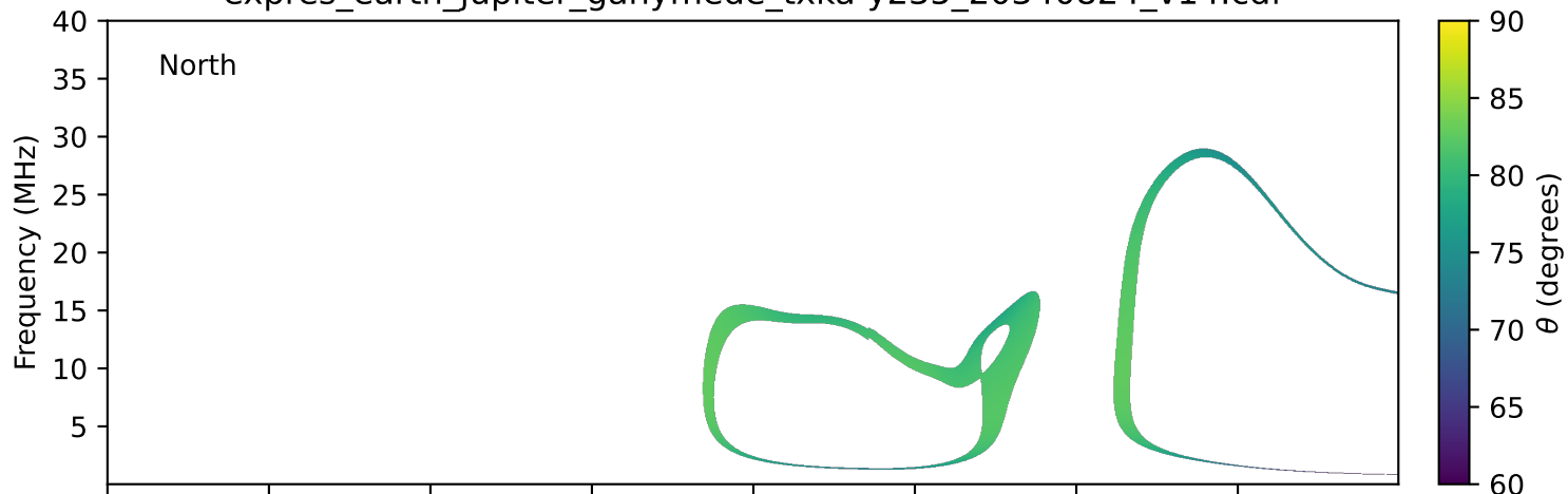
expres_earth_jupiter_ganymede_txka-y235_20340824_v14.cdf
