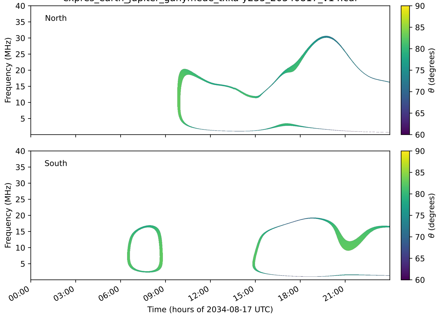
expres_earth_jupiter_ganymede_txka-y235_20340817_v14.cdf
