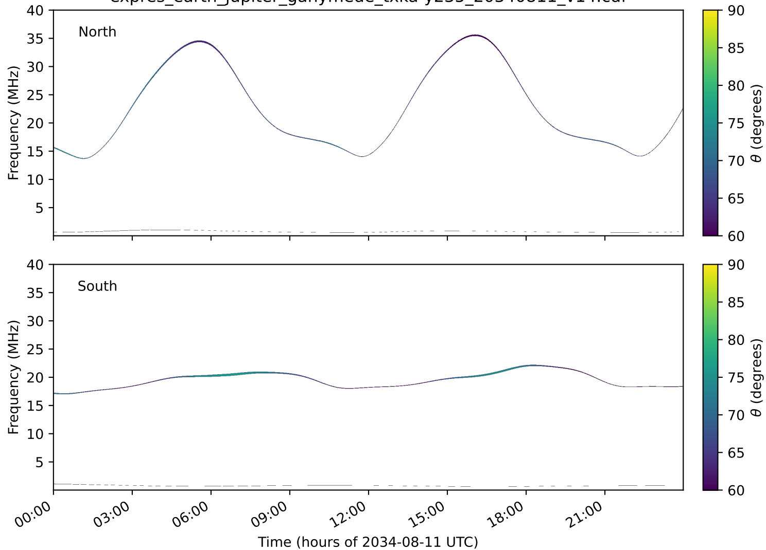
expres_earth_jupiter_ganymede_txka-y235_20340811_v14.cdf
