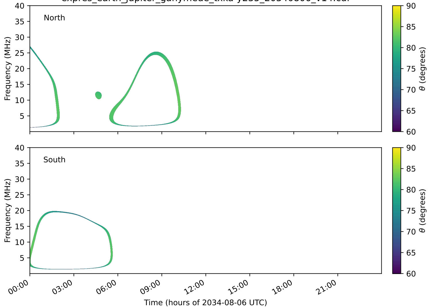
expres_earth_jupiter_ganymede_txka-y235_20340806_v14.cdf
