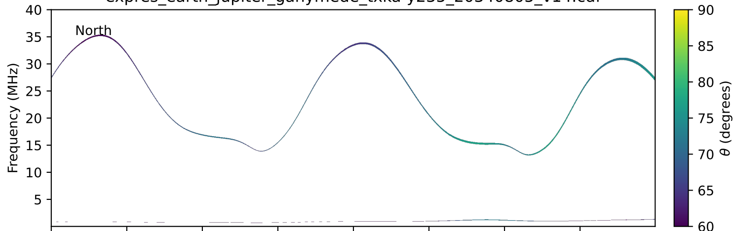
expres_earth_jupiter_ganymede_txka-y235_20340805_v14.cdf
