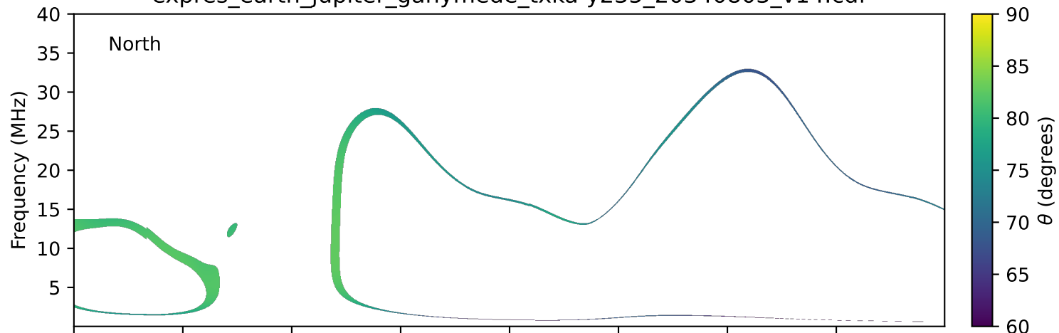
expres_earth_jupiter_ganymede_txka-y235_20340803_v14.cdf
