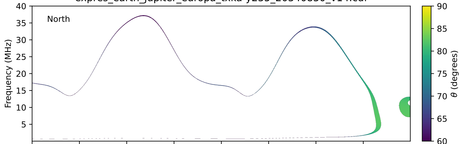
expres_earth_jupiter_europa_txka-y235_20340830_v14.cdf
