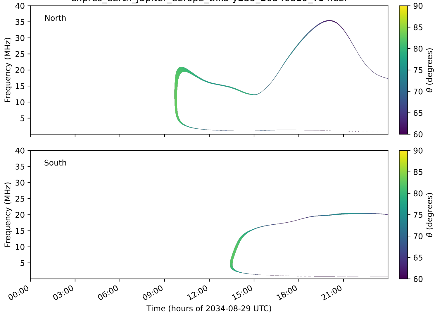
expres_earth_jupiter_europa_txka-y235_20340829_v14.cdf
