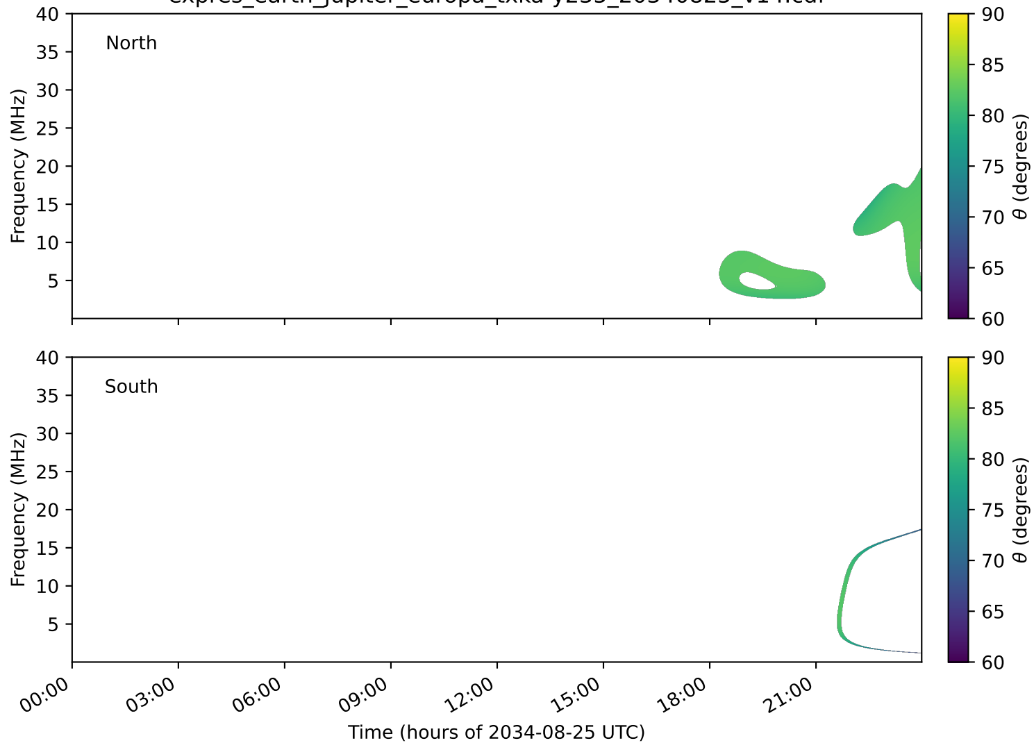
expres_earth_jupiter_europa_txka-y235_20340825_v14.cdf
