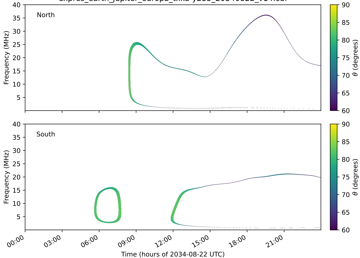
expres_earth_jupiter_europa_txka-y235_20340822_v14.cdf
