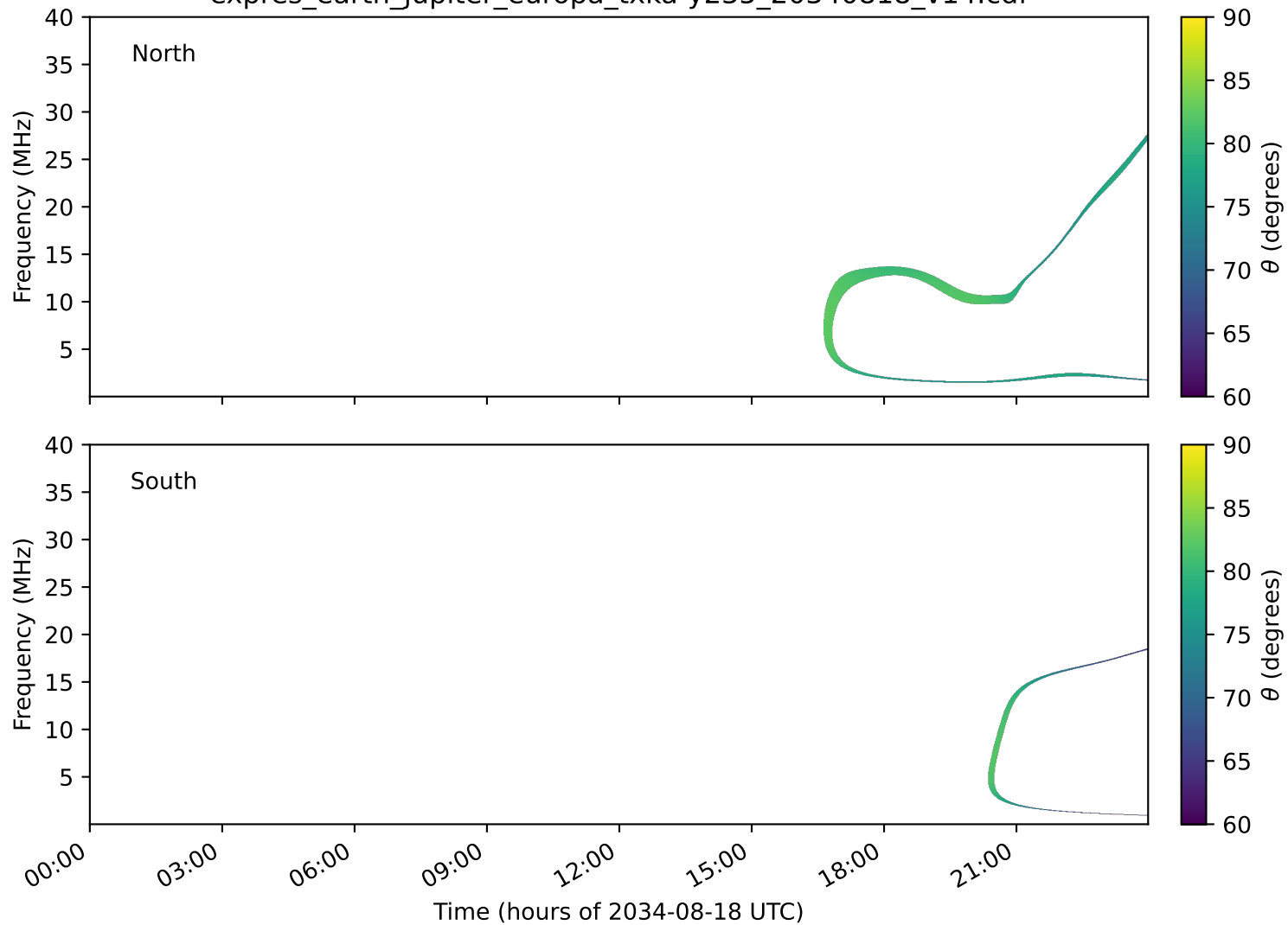
expres_earth_jupiter_europa_txka-y235_20340818_v14.cdf
