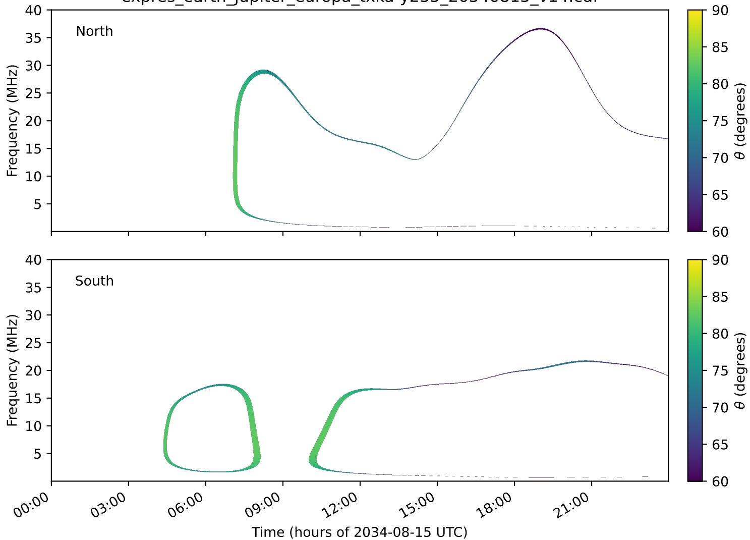
expres_earth_jupiter_europa_txka-y235_20340815_v14.cdf
